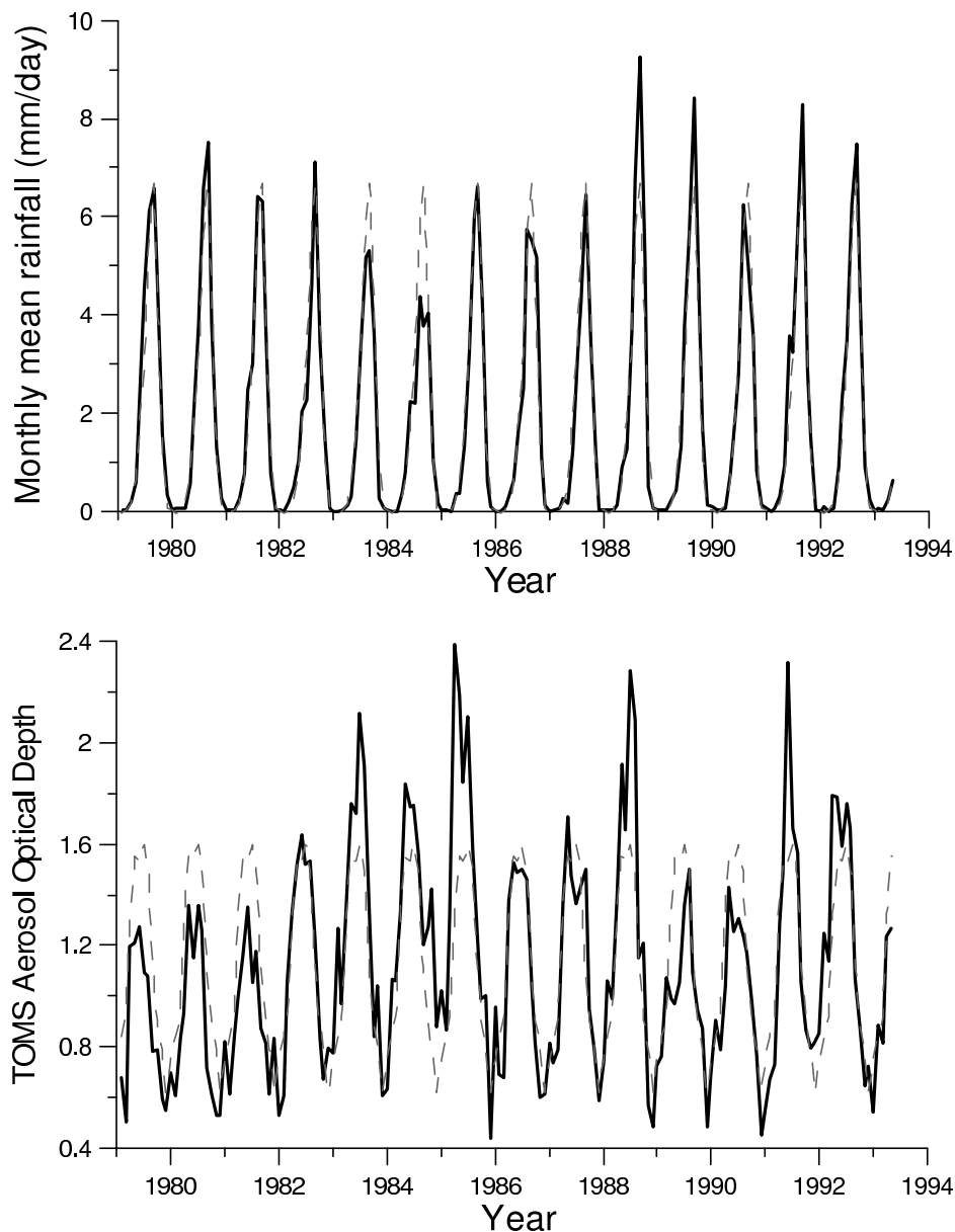
Figure 1. Monthly mean satellite-derived (a) GPCP precipitation [ \text{mm d}^{-1} ] and (b) TOMS dust Aerosol Optical Depth over the Eastern Sahel from 1/79–4/93. Solid lines are original data and dashed lines are fitted seasonal cycles.
