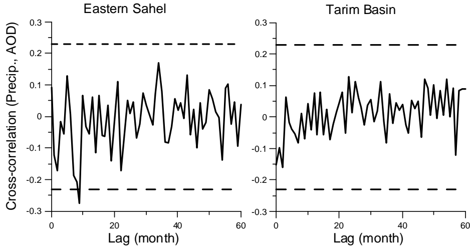
Figure 2. Lag cross-correlation of autoregression-corrected monthly mean seasonal precipitation and dust AOD anomalies over the (a) Eastern Sahel and (b) Tarim Basin. Confidence levels with p < 0.01 are at \pm 0.23 , shown as dashed lines.
