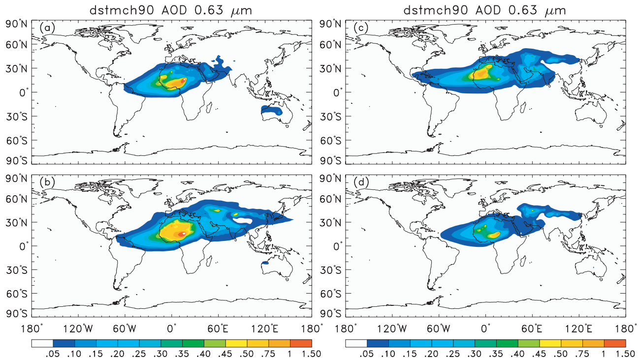
Figure 5. Predicted seasonal mean dust optical depth at 0.63 μm for (a) DJF, (b) MAM, (c) JJA, and (d) SON.
